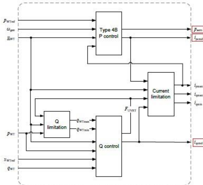
Fig. 29: Modular structure for the type 4b control model [1].
