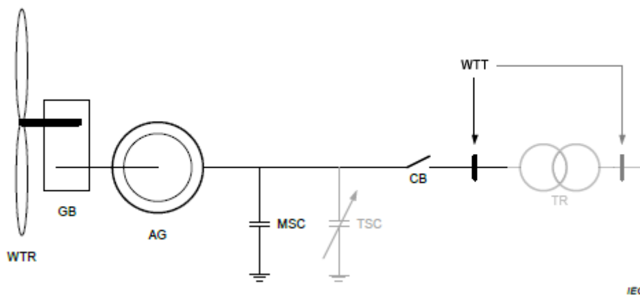
Fig. 1: Main electrical and mechanical components of type 1 WTs [1].
