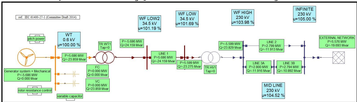
Fig. 9: System description type 2 WT
