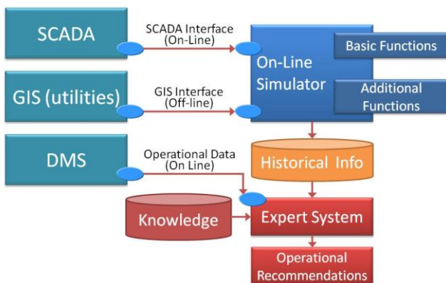
Fig.1. On-Line Simulator - Logical architecture.
